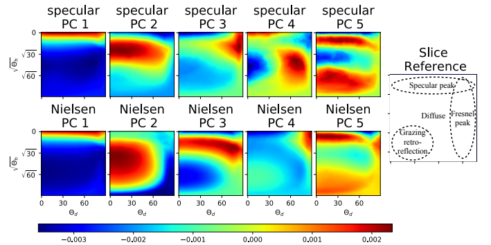
Fig. 12. Comparison of the BRDF slices of the specular principal components using our method and Nielsen et al. 's. We don't need a principal component to model the diffuse part like the second component of Nielsen et al. 's, thus our method yields more compact results.
