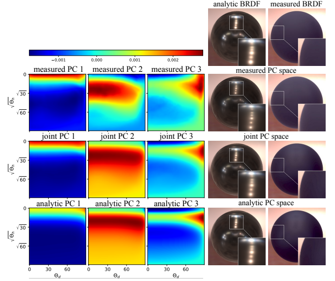
Fig. 16. The first three principal components trained from solely measured BRDFs in MERL dataset (second row), from analytic and measured BRDFs together (third row), and from solely analytic BRDFs (last row). We also compare the reconstruction results under these three spaces. By including analytic BRDFs into training, we can better recover the appearances of analytic BRDFs (fourth column), while still keeping the fidelity of measured BRDFs (last column).
