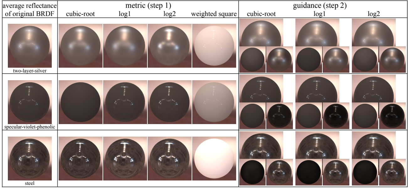
Fig. 3. The results of the first two steps of our separation algorithm. In step 1, we found that the weighted-square metric can't produce faithful results, and none of the other three metrics (cubic-root, log1, log2) performs consistently well on all BRDFs. However, the fitting results of all these three metrics leads to good separations in step 2. We choose to use the log2 metric in the following since it produces shorter tails on the specular parts. Note that we are working only on achromatic reflectances in this step.
