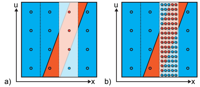
Figure 2: a) A slice through an XU light field showing an out-of-focus foreground object (orange) on an out-of-focus background (blue). Vertical dashed lines denote pixel boundaries, and disks denote input samples over the screen and lens. A traditional distribution ray tracer generates an image by averaging the input samples in a pixel. b) The light field, reconstructed at a large number of reconstruction locations by our algorithm. Thanks to the increased resolution, the resulting image is of much higher quality. A regular sampling is shown for clarity only; our algorithm operates on stochastic samples.
