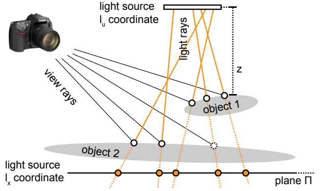
Figure 8: To reconstruct shadows from area light sources, we first determine the points that are visible from camera (black rays). We shoot a ray from a point on the light source (parameterized by l_u, l_v ) towards these points, and compute light-space depths z for the nearest hits as seen from the light. For shadowed view samples (dashed disk), the depth denotes the first occluder along the ray. The direction of light rays is parameterized by the l_x, l_y coordinates of their intersection with the \Pi plane.
