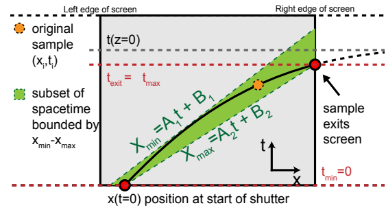
Figure 18: Bounding the reprojection of a sample. (See text.)
